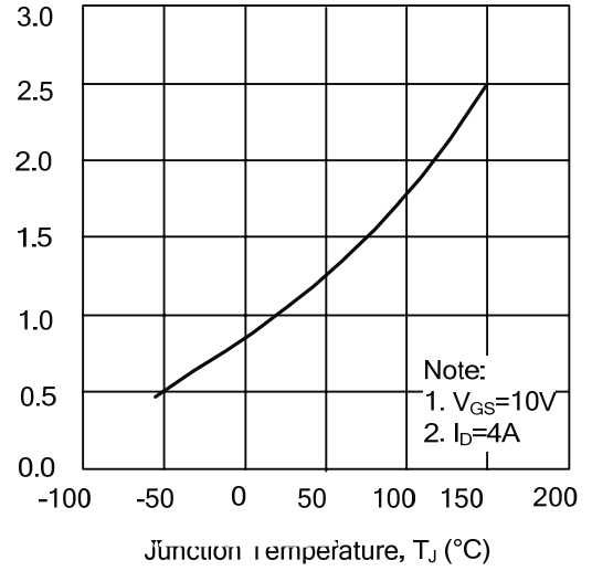
On-Resistance Variation vs. Junction Temperature
