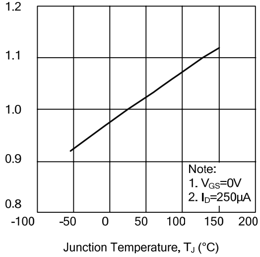
Breakdown Voltage Variation vs. Junction Temperature
